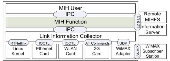
Fig. 2. Architecture of a GNU/Linux IEEE 802.21 prototype implementation
