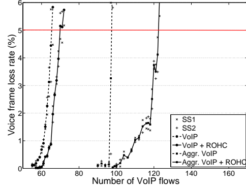
Figure 4. Voice frame loss
