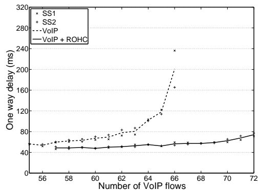
Figure 5. VoIP e2e OWD with & without ROHC
