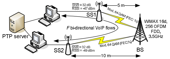
Figure 1. Schematic of the WiMAX testbed
