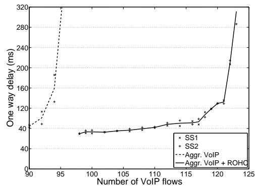
Figure 6. Aggregated VoIP e2e OWD with & without ROHC
